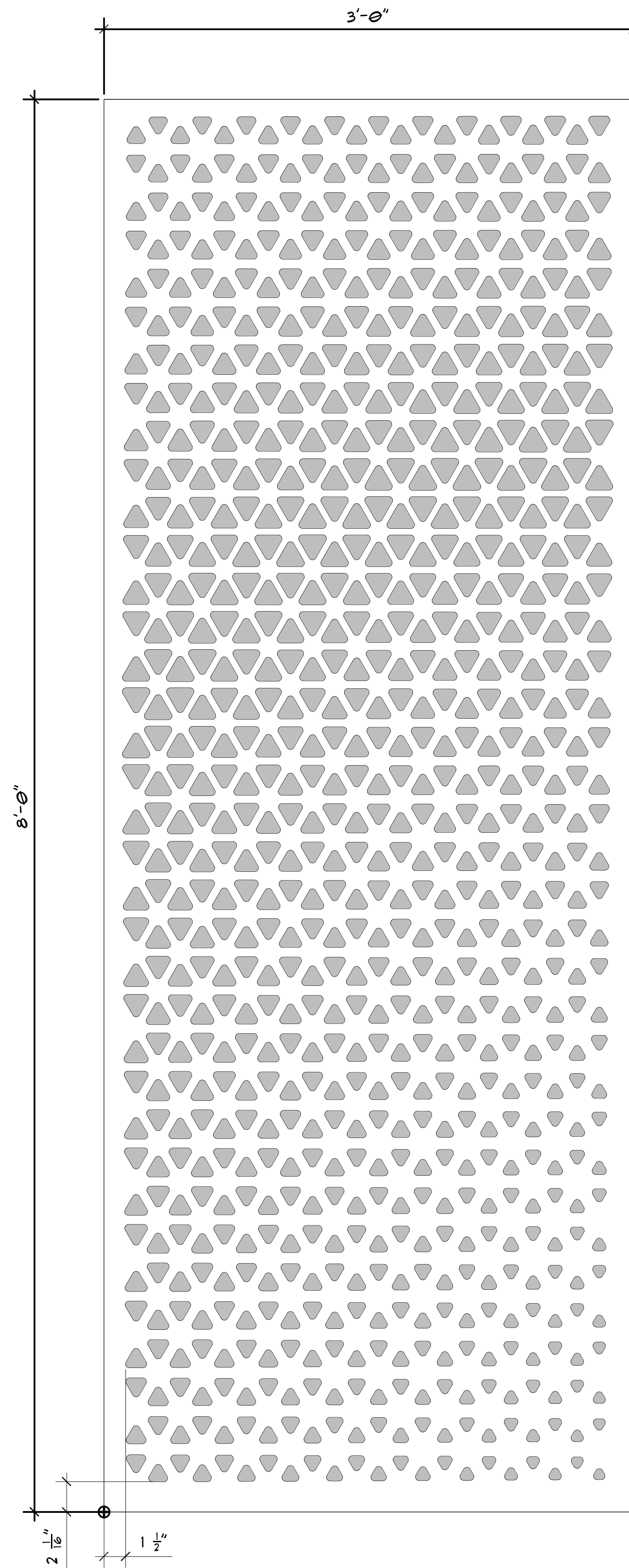
TRIGRID_PANEL_01.DXF
