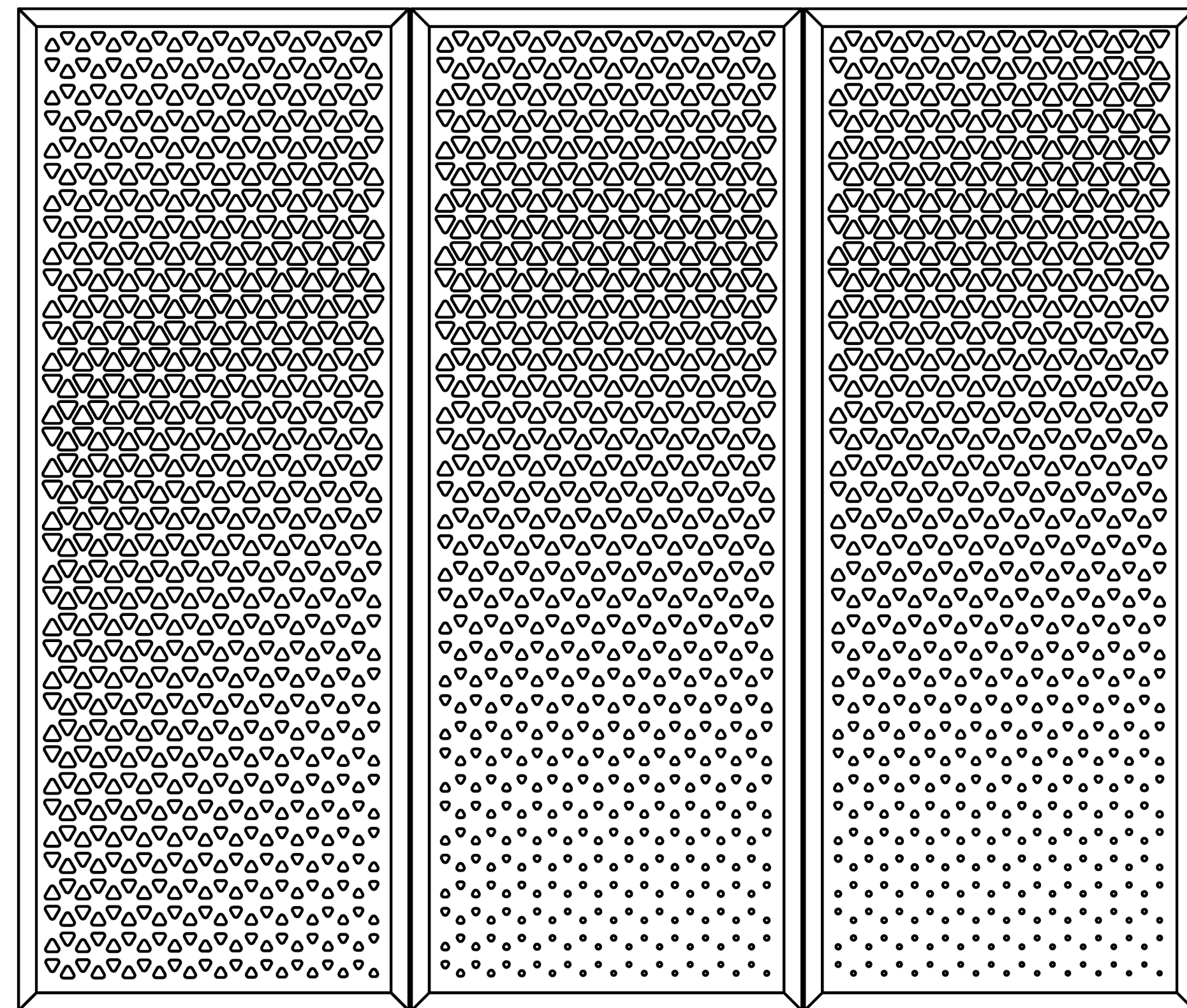
C ASSEMBLY DIAGRAM SCALE 1:12 1"=1'
