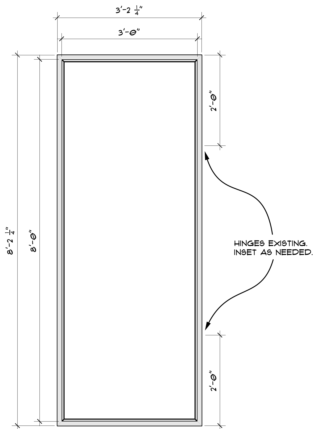
A FRAME SECTION SCALE 1:12 1"=1'
